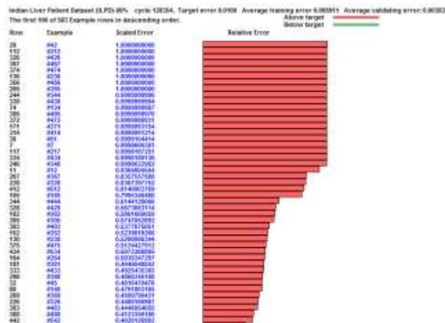
Figure 14: Errors in our ANN model of our proposed Liver Patient system
