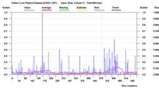
Figure 3: Data analysis with respect to Total Bilirubin
