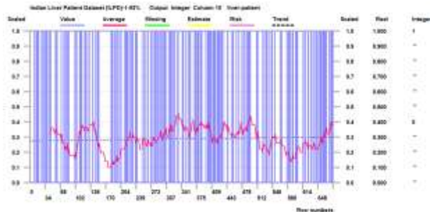
Figure 10: Data analysis with respect to Status
