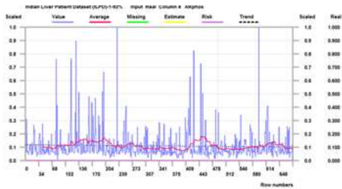
Figure 5: Data analysis with respect to Alkphos Alkaline Phosphatase
