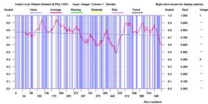
Figure 2: Data analysis with respect to Gender
