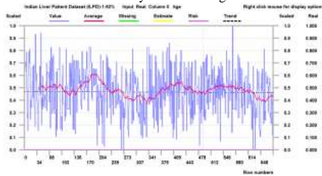
Figure 1: Data analysis with respect to Age
