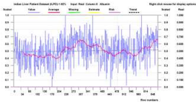
Figure 8: Data analysis with respect to Albumin
