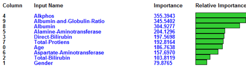
Figure 13: Most relevant factors in our ANN model of our proposed Liver Patient system
