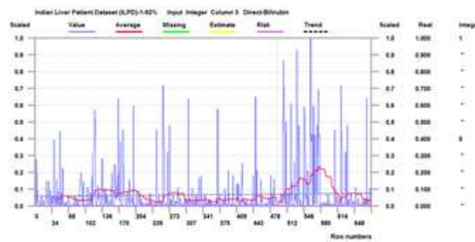
Figure 4: Data analysis with respect to Direct Bilirubin
